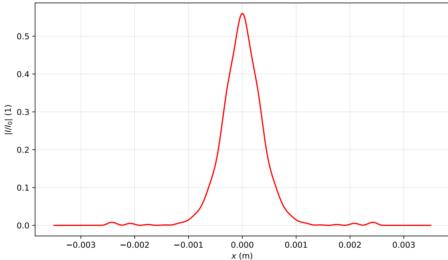
Intensity profile I(x, y = 0, z = 2.229)/I_0 , P_{in}=1.0P_{cr} , artificial time
